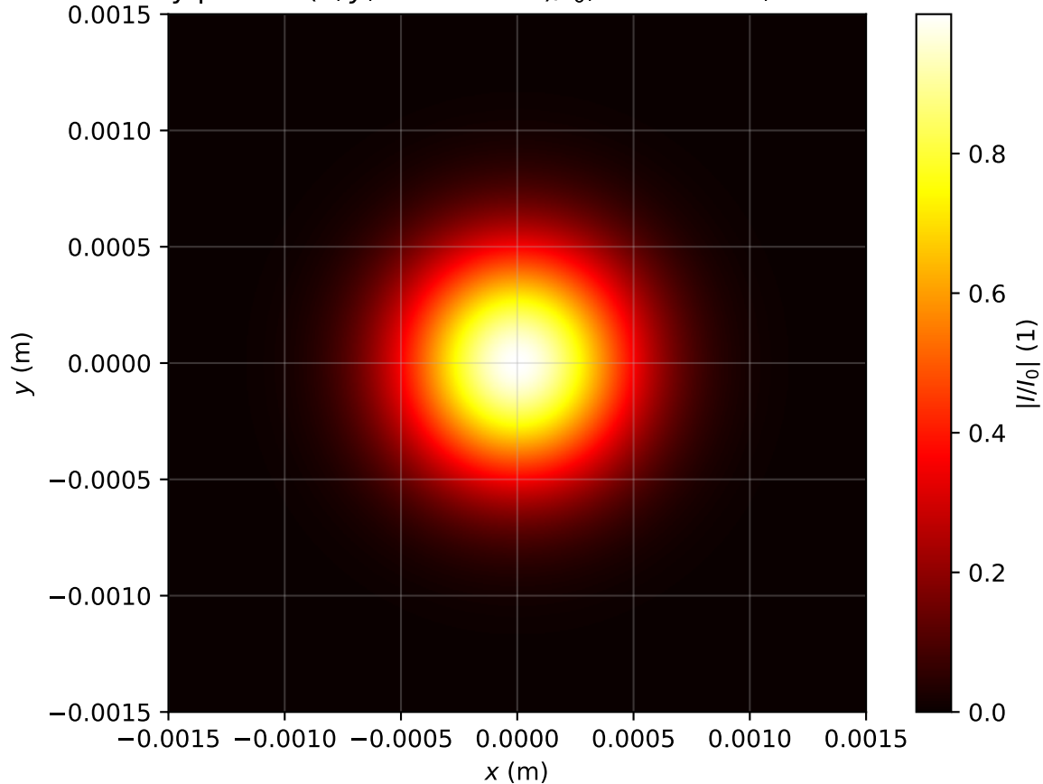
Intensity profile I(x, y, z = 0.080\text{m})/I_0 , P_{\text{in}}=0.2P_{\text{cr}} , artificial time
